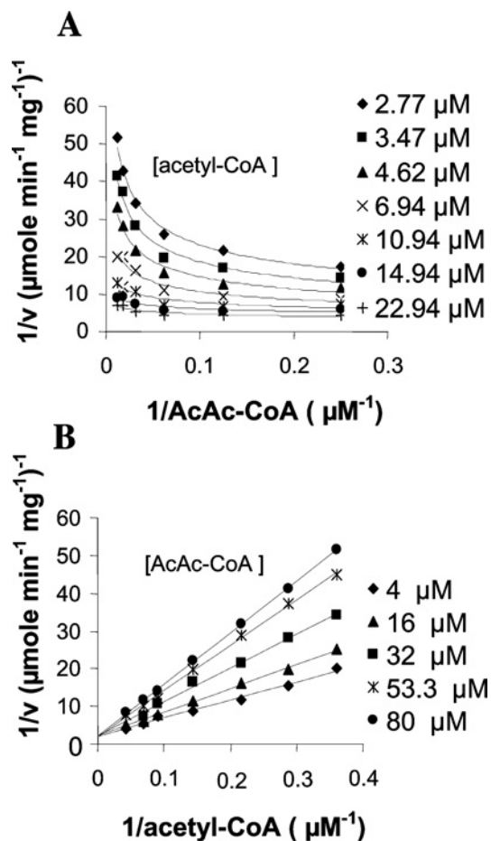
Figure 3 Determination of kinetic constants for His 6 -BjHMGS1
